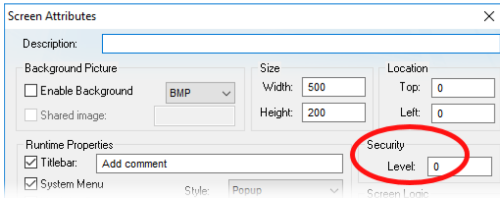
Security (access level) setting in Screen Attributes dialog
