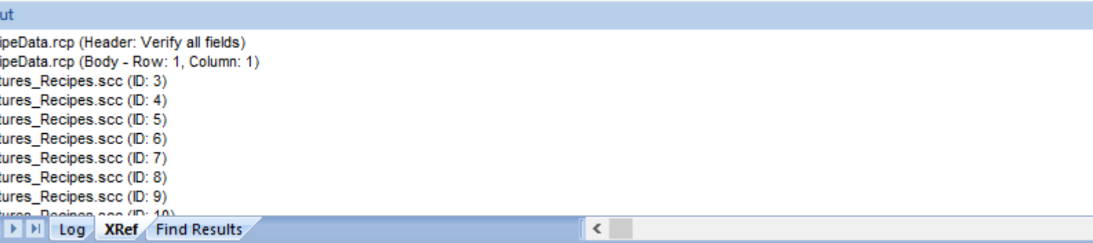
XRef Results
