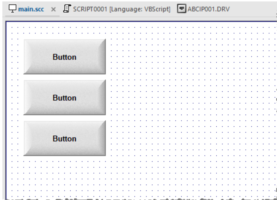
Screen/Worksheet Editor
