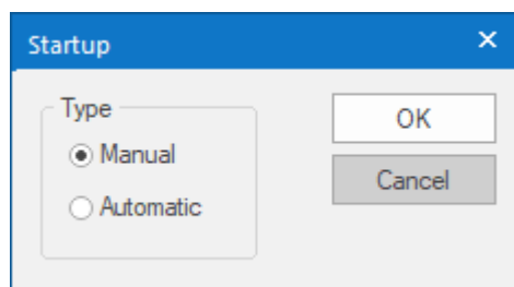
Startup dialog
