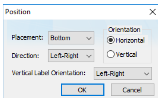
Position Dialog
