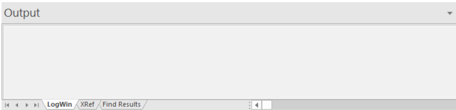
Output window
