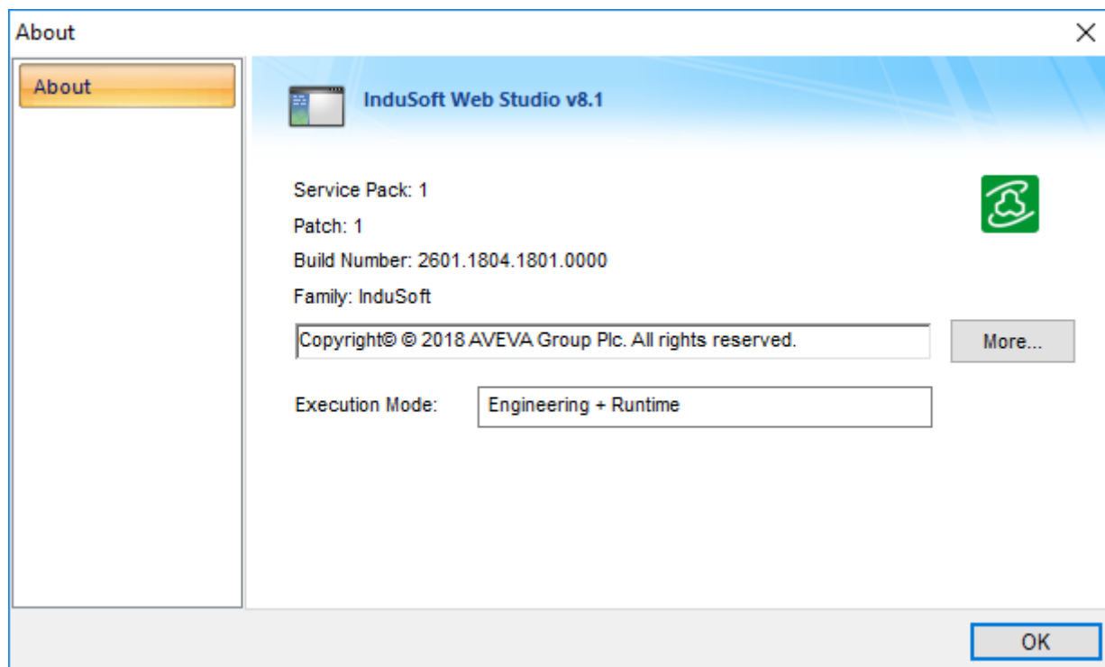
About dialog
