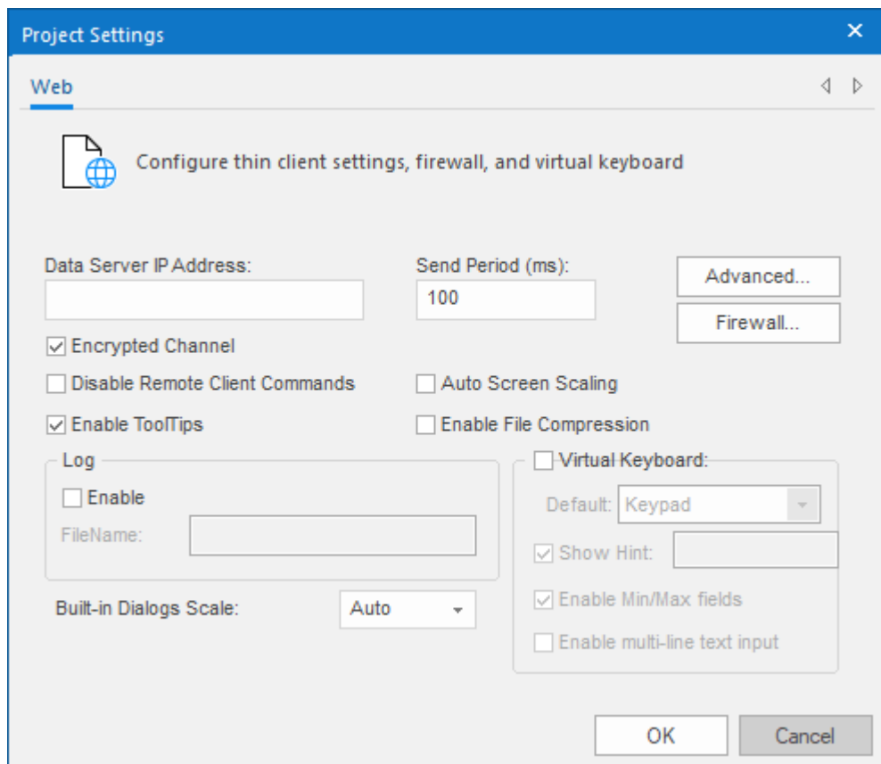
Web tab of Project Settings dialog
