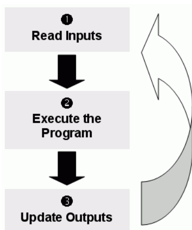
PLC Program Loop
