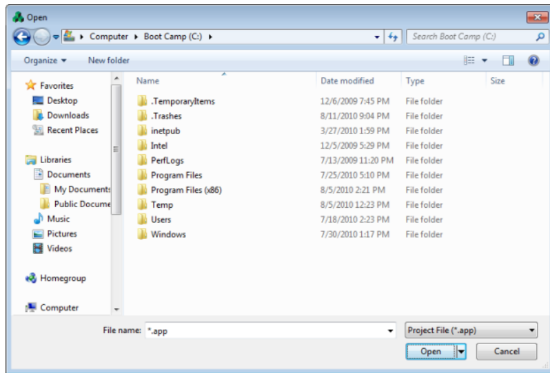
Open dialog
